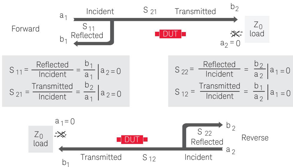
Figure 17. Measuring S-parameters
