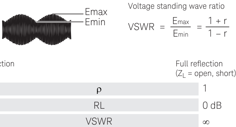
Figure 11. Reflection parameters
